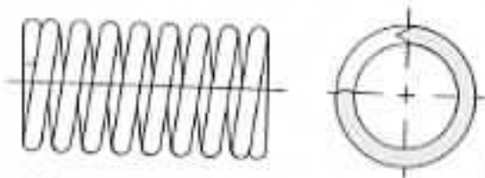
Closed, Squared and Ground Ends Coiled Left-hand
